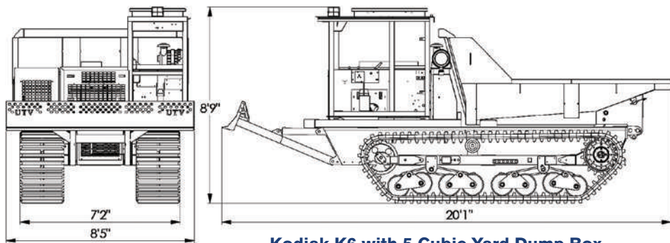
Kodiak K6 with 5 Cubic Yard Dump Box
